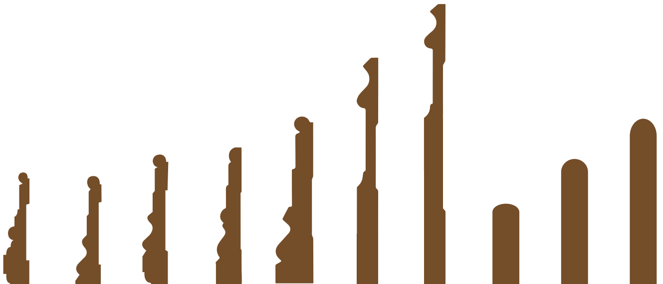
B74 95 x 22 Victorian B14 92 x 22 Old Colonial B18 110 x 22 Old Colonial B23 115 x 25 Old Colonial B75 140 x 32 Old Colonial B20 190 x 18 Old Colonial B21 235 x 18 Old Colonial B116 90 x 32 Nosing B117 140 x 32 Nosing B118 185 x 42 Nosing
